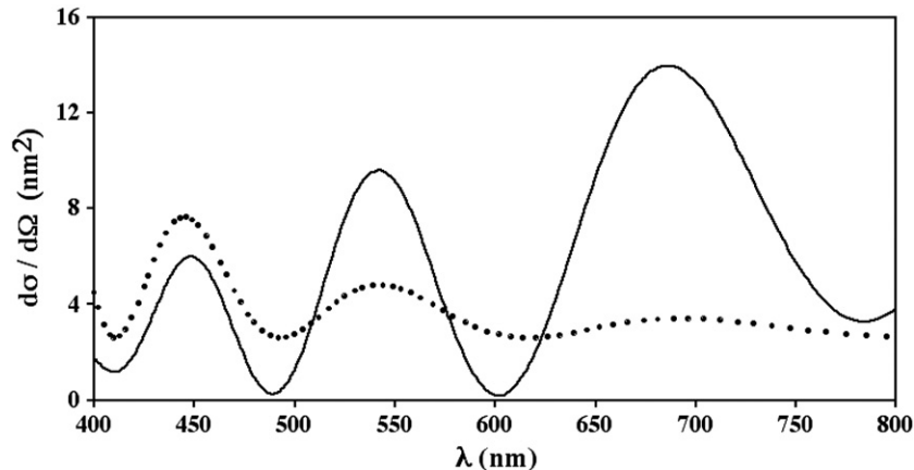
Fig. 3. Differential cross-sections of scattering for spherical:— continuous line, and ellipsoidal pores:— dotted line; sphere radius: = 3.6 nm and mean spacing c=8 nm ellipsoid: long axis=3.6 nm, short axis=3.4 nm and mean spacing c=6.9 nm.
