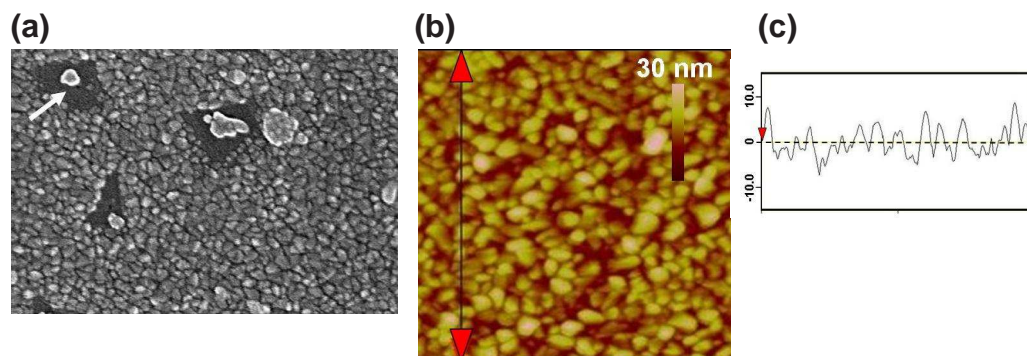
Fig. 1. R–SnO 2 morphology (a) SEM image: holes are present in the coating (cf. arrow) (b–c) AFM image (0.25 μm 2 ) and corresponding section profile.
