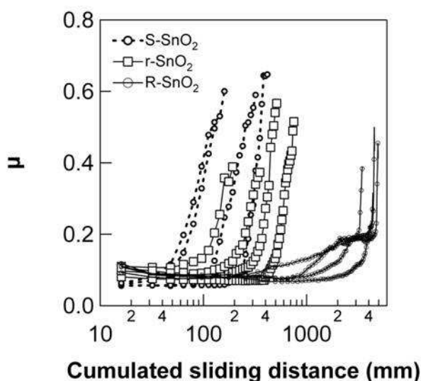
Fig. 12. Evolution of \mu with the cumulated sliding distance when the polymer is deposited on (---○---) \text{S-SnO}_2 , (—□—) \text{r-SnO}_2 and (—○—) \text{R-SnO}_2 . \mu averaged on the first cycle is: 0.06 for \text{S-SnO}_2 and 0.09 for \text{r-SnO}_2 .
