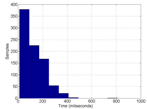
Figure 14. Computation time histogram for the complete sequence
