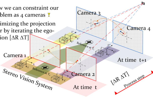
Figure 4. Trifocal constraints
