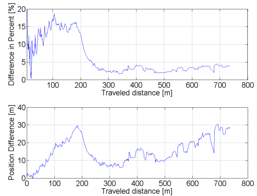
Figure 11. Difference evolution between GPS and Visual Odometry
