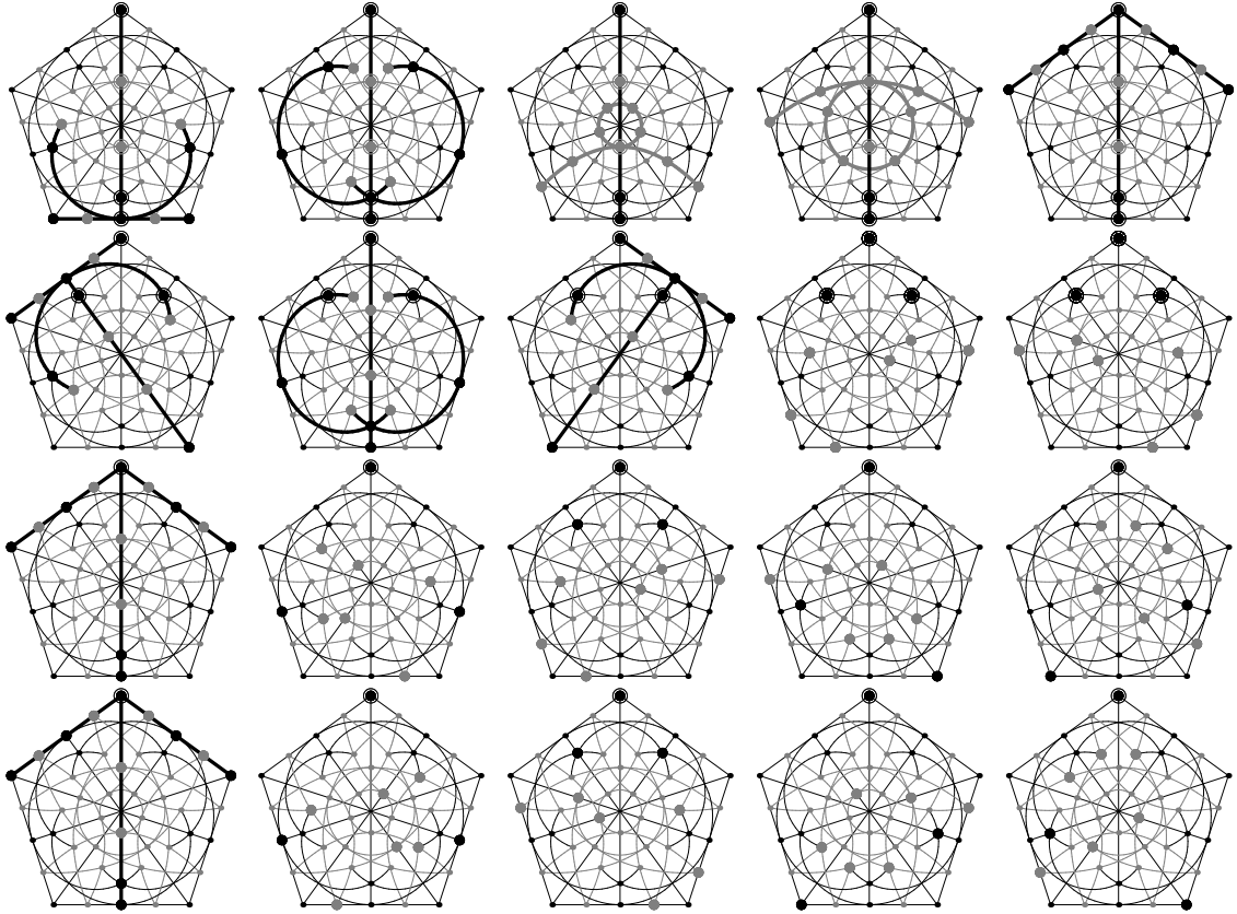
Figure 2: Representatives of the four different types of V-lines forming the linear subspace of \mathcal{V}(\text{GQ}(4, 2)) isomorphic to \text{PG}(3, 4) . The encircled bullets represent the points shared by all the five V-points forming a given V-line.
