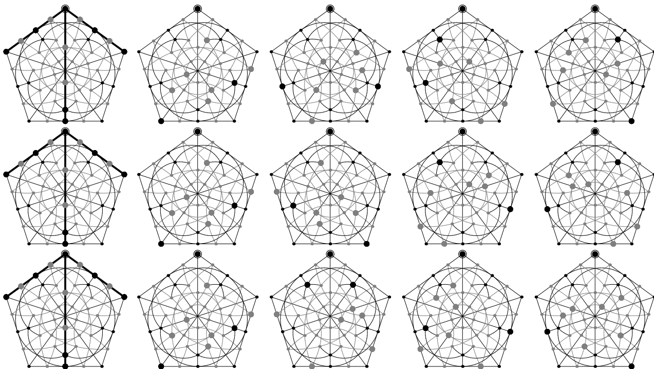
Figure 4: An example of three different V-lines on two common V-points (a perp and a (tri-)tripod).
