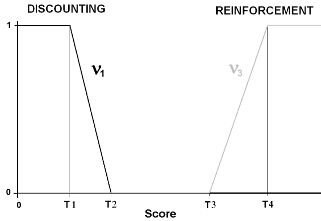
Figure 10: Coefficients \nu_1 and \nu_3 as functions of the score. The three coefficients \nu_1 , \nu_2 and \nu_3 are linked by the equation \nu_1 + \nu_2 + \nu_3 = 1 .
