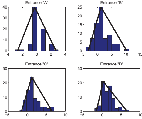
Figure 3: Empirical distributions of error counts for the entrances of the junction
