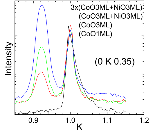
Figure 3: Surface X-ray diffraction pattern during the growth of the \text{NiO}/\text{CoO} mixed oxide over the \text{PtCo}(111) surface alloy
