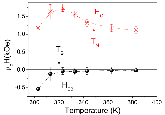
Figure 7: Exchange bias shift (circles-black) and coercivity (stars-red) as function of temperature. The blocking temperature T_B is estimated at 320 K, close to the maximum coercivity.
