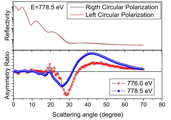
Figure 8: XRMS at the Co L_3 edge. Upper curves correspond to the two polarizations at E=778.5 . The curves display the asymmetry ratio at two different energies about the edge.
