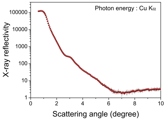
Figure 4: X ray reflectivity ( \text{Cu } K_{\alpha} , \lambda = 0.154 \text{ nm} ) measurements from the rough oxide surface. The surface has a large roughness, 1 nm, while the interface is quite flat, with roughness of about 0.1 nm.
