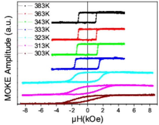
Figure 6: PMOKE hysteresis loops measured at different temperatures, after field cooling from 400 K under 5 kOe.
