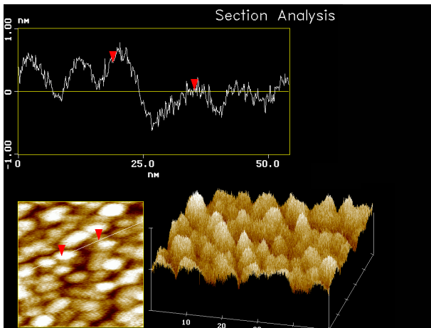
Figure 5: AFM of a 12 ML CoO layer grown by electron beam evaporation on top of a Pt(111) single crystal. A roughness close to 1 nm can be observed
