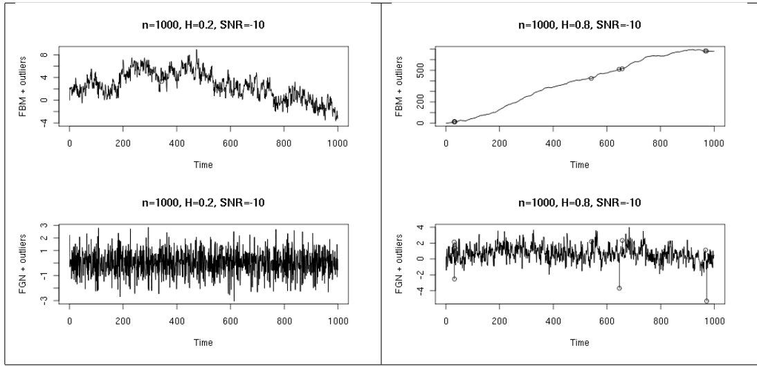
Figure 5: Example of contaminated fractional Brownian motions (model AO with a SNR = -10 ) with Hurst parameters H = 0.2 (left) and H = 0.8 (right) and length n = 1000 .
