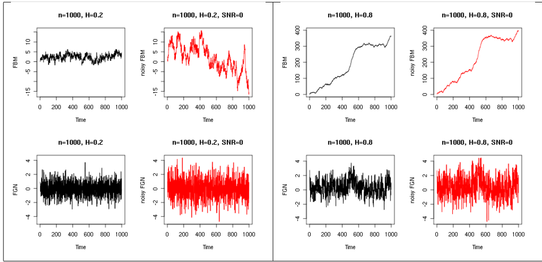
Figure 9: Example of a contaminated fractional Brownian motion (model B0 with a SNR = 0 ) with Hurst parameters H = 0.2 (left) and H = 0.8 (right) and length n = 1000 .
