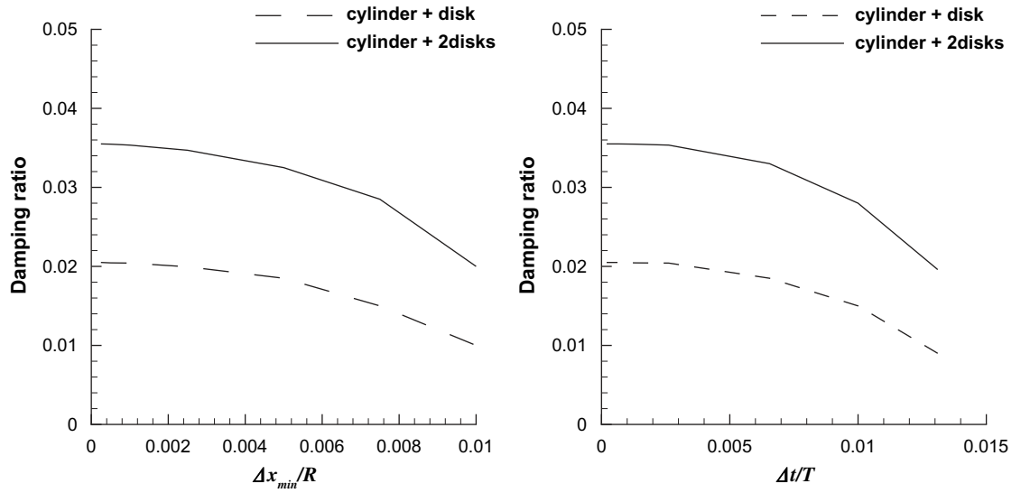
Fig. 3. Convergence tests.
