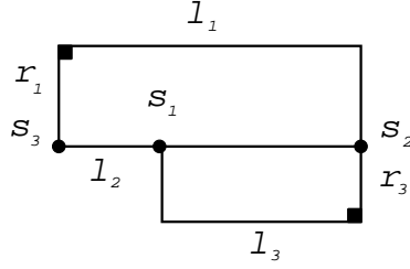
Figure 14: Permitted gluing of two rectangles
