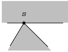
Two rectangles are degenerate
