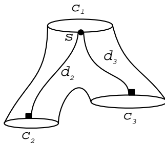
Figure 7: Singularity on the boundary
