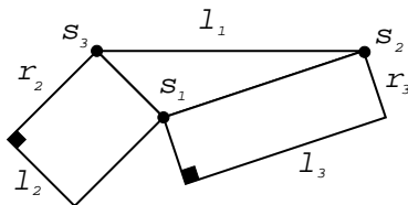
Figure 8: The resulting heptagon after cut
