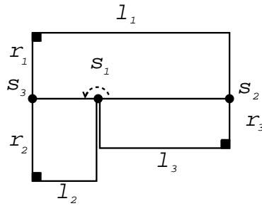
Figure 5: Here we see the triangle on the pair of pants
