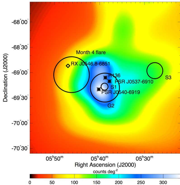
Figure 2: Zoom into a 3^\circ \times 3^\circ large region of the background subtracted counts map around the central star cluster R 136 in 30 Dor. Stars show the locations of R 136 and of the pulsars PSR J0540–6919 and PSR J0537–6910. The circles show the 95% containment radius of sources S1 and S3 of the point source model, and of source G2 of the 2D Gaussian shaped model (see text). During month 4 of our dataset, a flaring point source occurred near 30 Dor, and we indicate the 95% containment radius of this source; the diamond shows the location of the possible counterpart RX J0546.8–6851 of the flaring source.
