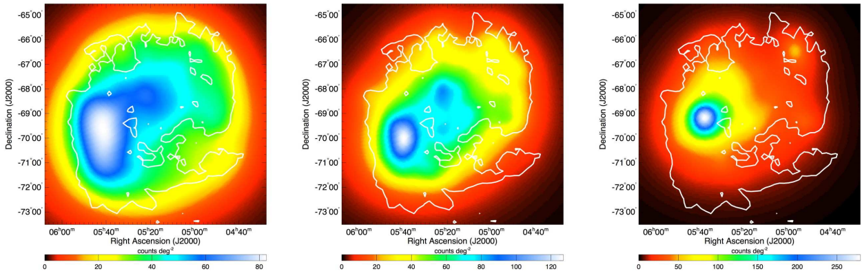
Figure 4: Gas tracer maps convolved with the LAT point spread function and scaled using maximum likelihood model fitting to the data. Panels show HI (left panel), H 2 (mid panel), and HII (right panel).
