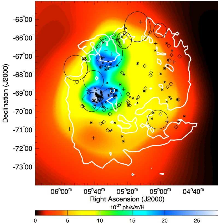
Figure 6: Integrated > 100 MeV emissivity maps of the LMC in units of 10^{-27} \text{ ph s}^{-1} \text{ sr}^{-1} \text{ H-atom}^{-1} . An adaptive smoothing with a signal-to-noise ratio of 5 has been applied to reduce statistical fluctuations. The white line shows the N(\text{H I}) = 10^{21} \text{ H cm}^{-2} iso column density contour to indicate the extent of the gaseous disk. Symbols indicate the locations of pulsars (pluses) from ATNF catalogue version 1.36 [24], supernova remnants (diamonds) from Rosa Williams web page http://www.astro.illinois.edu/projects/atlas/index.html , Wolf-Rayet stars (stars) from the fourth catalogue of [25], and supergiant shells (circles) from [26].
