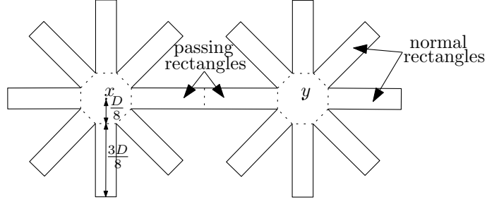
Figure 2: Polygon \mathcal{P}
