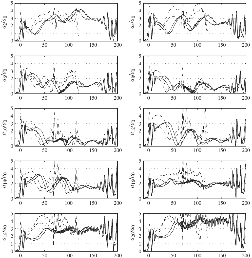
FIGURE 16. Wave period 1.13s. Steepness H/L=4\% . Time evolutions of the measured free-surface elevations RAOs at every other gauge from arrival of the wavefront. The solid line denotes CEHIPAR experiments and the dashed line denotes BGO-First experiments. (Horizontal scale is non-dimensional time t/T , T being the wave period.)
