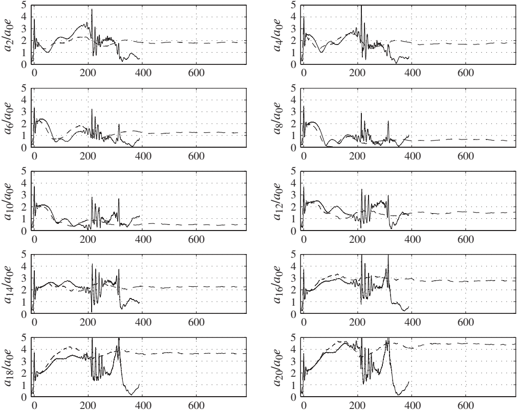
FIGURE 21. Wave period 1.13 s. Steepness H/L=3\% . Time evolutions of the free-surface elevations RAOs at every other gauge from measurements (solid line) and the Boussinesq model (dashed line).
