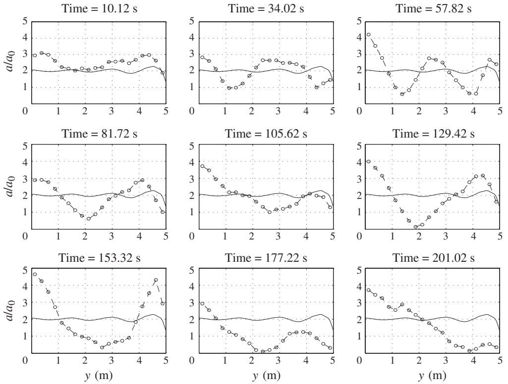
FIGURE 12. Wave period 1.01 s. Steepness H/L=4\% . Time evolution of the free-surface elevation RAO along the plate from experiments ( \circ ) and linear theory (solid line). Plate moved at 75 m from the wavemaker.
