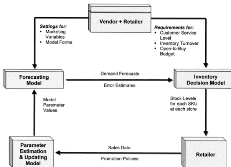
Figure 1: Models used for VMI Decision Support System [Achabal et al, 2000]
