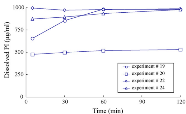
Fig. 8. Dissolution rate profiles for different SCF processed samples.
