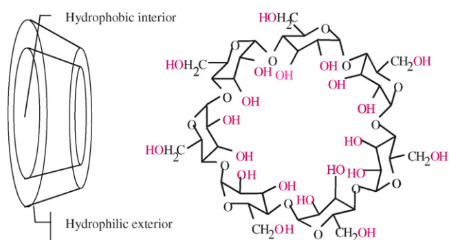
Fig. 1. Formula of \beta -cyclodextrin.
