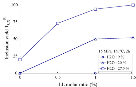
Fig. 4. Inclusion yield T_{CX}^{PI} vs. LL molar ratio for different water contents.
