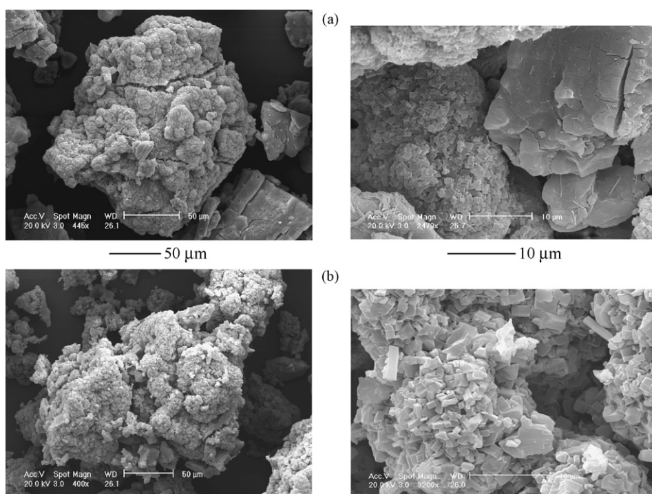
Fig. 6. SEM pictures of partially (a) and completely (b) complexed powders.
