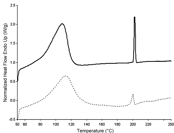
Fig. 3. Typical DSC curves: physical mixture (solid line) and SCF processed sample (dashed line).
