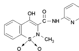
Fig. 2. Formula of piroxicam.
