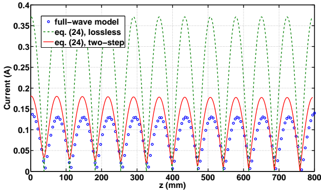
Fig. 5. The current distribution along the overhead wire for the example in Fig. 4, as computed at the TRP peak at f = 2.029 GHz.
