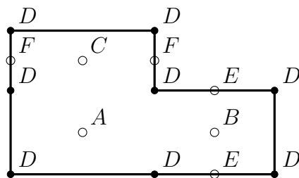
FIGURE 2. Weierstrass points
