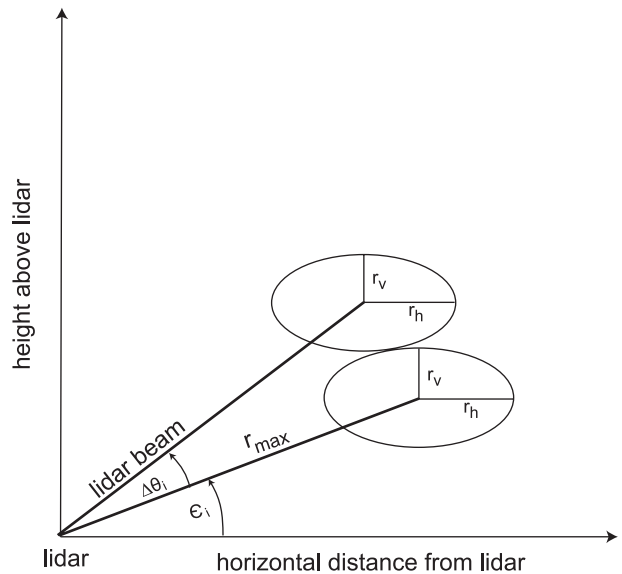
FIG. 6. Ellipsoids with half axes determined by the radii of influence r_v and r_h at two (vertical) successive beams touch each other at the distance r_{\max} . The lower beam is at elevation angle \epsilon_i , with elevation step \Delta\theta_i to the upper beam.
