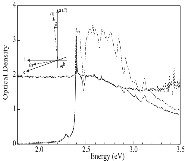
FIG. 5: Absorption spectra, at 13 K, of a crystal with x_p \sim 1.4 \times 10^{-3} for different configurations of the polarizer and analyzer. Dash-dotted line: // configuration; solid line: // (no analyzer) configuration; dots: // - \perp configuration. Inset: geometrical configuration for absorption spectroscopy of 3NPh2 crystals. a , b , c are the crystallographic axis. (1) and (2) are two of the principal axis of [\epsilon_1] ; b is the third principal direction in a monoclinic crystal. \delta is the angle between a and (1). In the experiments the incident light is perpendicular to the (a,c) plane and polarized either parallel ( // ) or perpendicular ( \perp ) to a .
