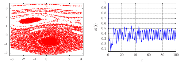
Figure 3: Left: “Poincaré section” of a QSS for E/N = 1.2 , N = 65536 . Initial conditions are Gaussian in p and q = 0 . The section is computed for 150 < t < 1000 and \alpha = 0.25 . Right: Magnetization versus time.
