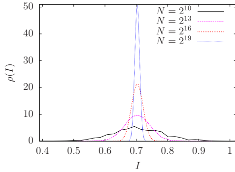
Figure 1: QSS for the \alpha -HMF model built using a stationary solution of the HMF model corresponding to a one particle PDF of the type f(I, \theta) = \delta(I - I_0)/2\pi (one torus M = 0.5 ). The system is evolved via the \alpha -HMF dynamics with \alpha = 0.25 . The figure displays the resulting distribution of actions I at t = 200 , for different sizes. The integration uses the fifth order optimal symplectic integrator [11] and a time step \delta t = 0.05 .
