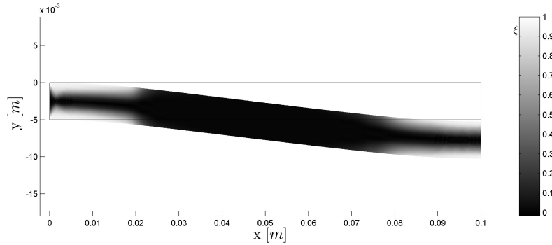
Figure 8. Martensite rate distribution at t = 1 ms (end of impact) for the isothermal configuration
