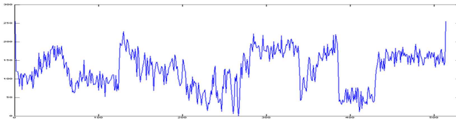
(b) Noisy slice
