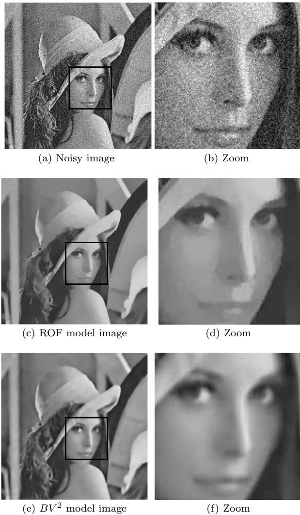
Fig. 11 Staircasing effect - \sigma = 0.25 , \lambda = 50 , 10 000 iterations.
