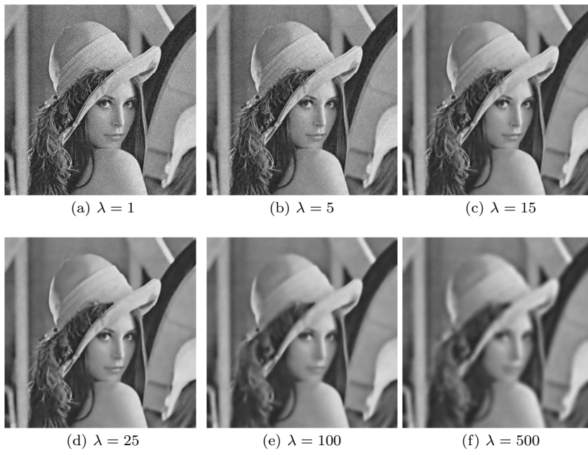
Fig. 3 Standard deviation \sigma = 0.15 - 5000 iterations
