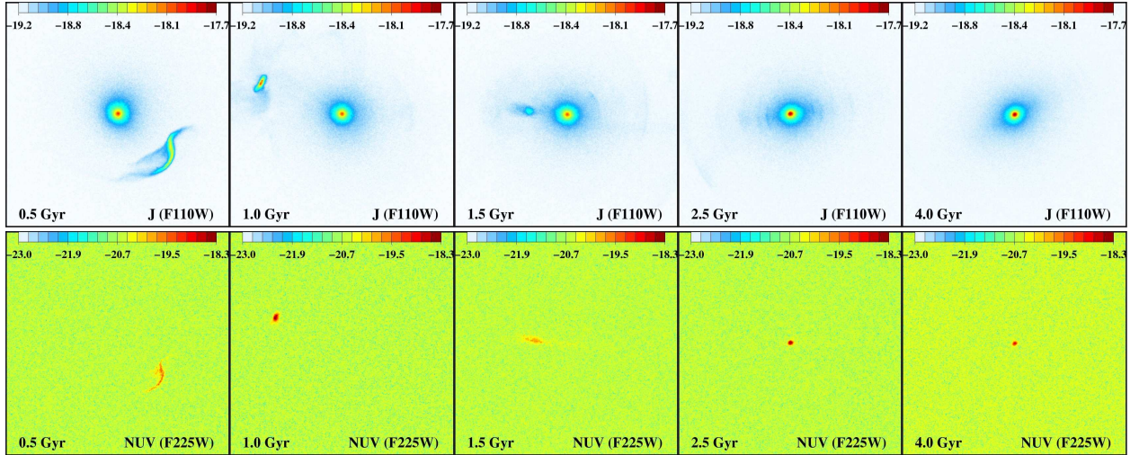
Figure 11. The evolution of synthetic images from experiment B_1 (mass ratio 1:6 and c_*=0.01 ) through J (first line) and NUV (second line) assuming the observed system at z \sim 0.023 .
