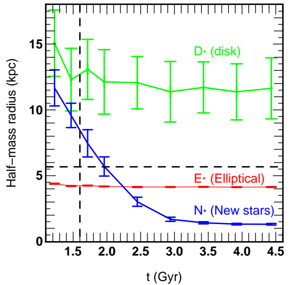
Figure 6. The upper panel shows the evolution of the half-mass radius (green line) and effective radius from V (blue) and H (red) bands for experiment B_2 . In the lower panel, we show the evolution of the half-mass radius for each stellar component: stars that initially belong to the host elliptical galaxy ( E_* , red line), those that were present in the disk before the merger ( D_* , green line) and the new stars which have been formed during the merger process ( N_* , blue line). In each panel, the horizontal dashed line is the predicted half-mass radius value after the merger from arguments based on the virial theorem whereas the vertical dashed line is the epoch of the final plunge.
