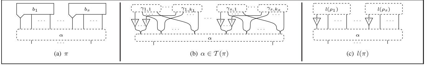
Figure 4: (a) an ll-net \pi s.t. \text{box}_0(\pi) = \{b_r\}_{r \leq s} ; (b) the generic shape of a simple net \alpha \in \mathcal{T}(\pi) ; (c) the linearization l(\pi) .
