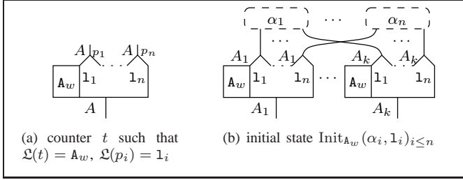
Figure 8: counter and initial state.
