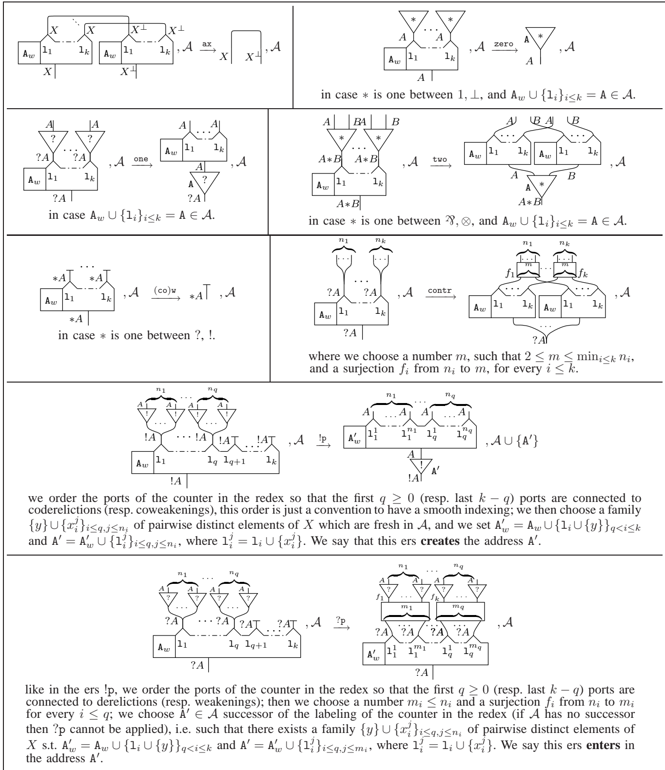
Figure 9: the elementary reduction steps (ers for short) of merging reduction; the net at left of an ers is the redex , the one at right is the contractum of the ers. In the ers contr , ?p , we present a bunch of contractions and wirings as a surjective function f from the auxiliary ports to the principal ones.
