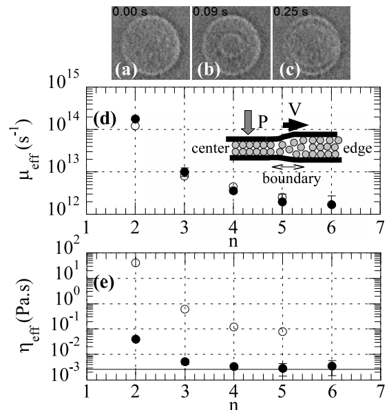
FIG. 3: (a-c): Sequence of images ( 96 \times 96 \mu\text{m}^2 ) showing the front propagation during a 3 \rightarrow 2 transition. (d): \mu_{\text{eff}} vs n (number of monolayers). ( \bullet ) our results, ( \circ ) BM results, adapted from [9]. Inset: schematic cross-section of the film during squeeze-out. (e): \eta_{\text{eff}} vs n . ( \circ ) measured in shear, and ( \bullet ) deduced from squeeze-out experiments. The horizontal line indicates the bulk viscosity of OMCTS.
