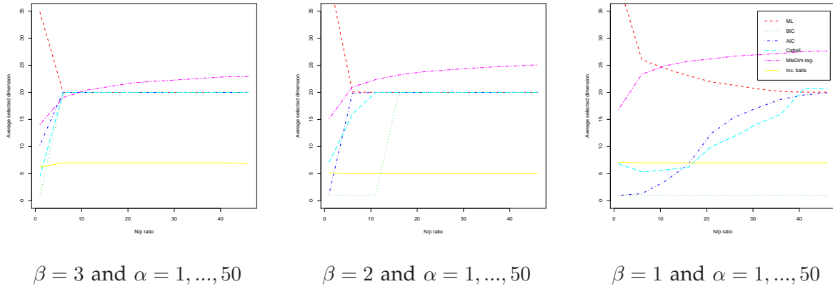
Fig. 5. Average selected dimension according to the ratio \alpha = n/p for different values of \beta with ML, AIC, BIC and the scree-test of Cattell. The data were simulated according to a uniform distribution (see text for details) with p = 50 and the actual intrinsic dimension is d^* = 20 .
