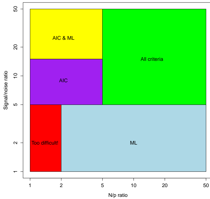
Fig. 6. Recommended criteria for intrinsic dimension selection according to the n/p and signal to noise ratios in the context of the isotropic PPCA model.
