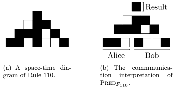
Figure 1: Problem \text{PRED}_{F_{110}} .
