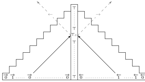
Figure 7: A CA easy for PRED and hard for INV
