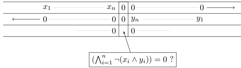
Figure 6: An automaton with a hard CYCLE problem, and an easy INV.
