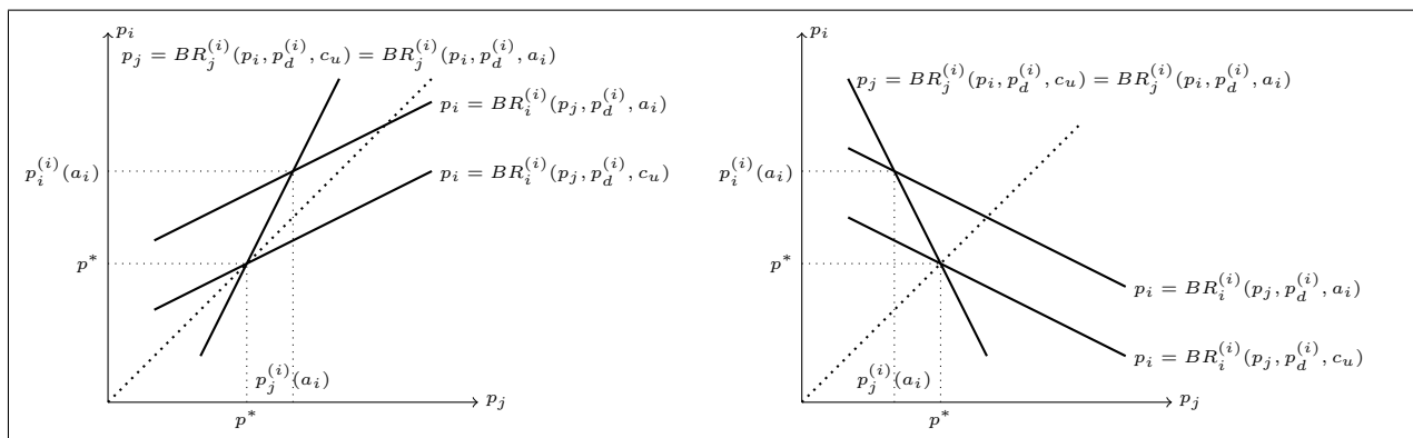
Figure 3: Graphical representation of the proof of Lemma 1
