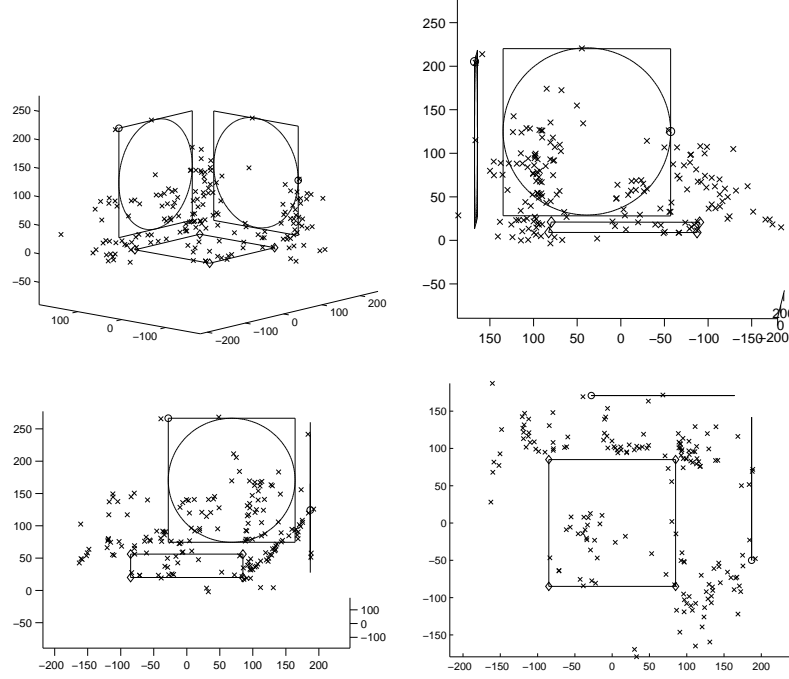
Fig. 7. Cloud of 3-D reconstructed points of the scene of Sequence 1. Legend : ' \diamond ' = known coplanar points, ' \circ ' = 3-D reference points, ' \times ' = reconstructed points
