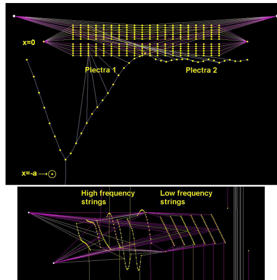
Figure 16: Two different viewpoints of the simulation of the model shown on the figure 13 at 2,5 seconds. Second phase of the period of the “macrostring” movement. This one goes up until it reaches the “ x=0 ” plan. So now the seven plectra of the second group pluck the high frequency strings as we can verify it on the bottom picture.
