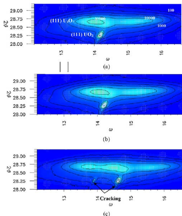
Figure 2: X-ray diffraction maps of a (1 1 1) surface of a UO_2 single crystal after an in situ oxidation treatment at 300 °C in air for (a) 1.5 h, (b) 3.5 h and (c) 10 h. The intensities (a.u.) are reported close to the level lines.
