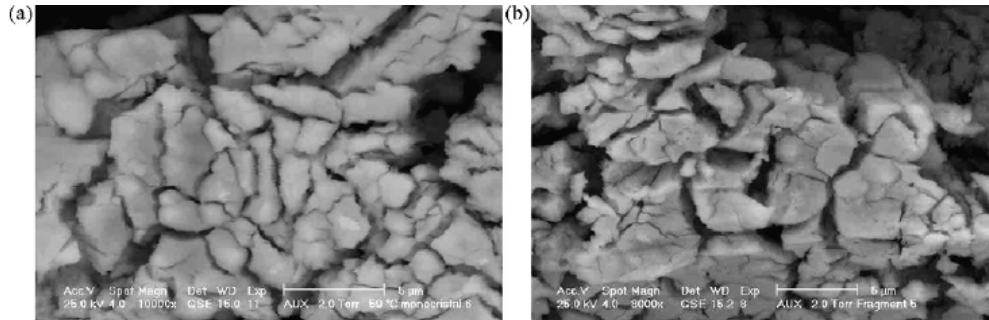
Figure 4: ESEM micrographs showing detailed areas of the subdivided final states of (a) UO 2 single crystal and (b) UO 2 fuel pellets oxidised for 5.5 h at 330 °C and P O 2 = 265 Pa.
