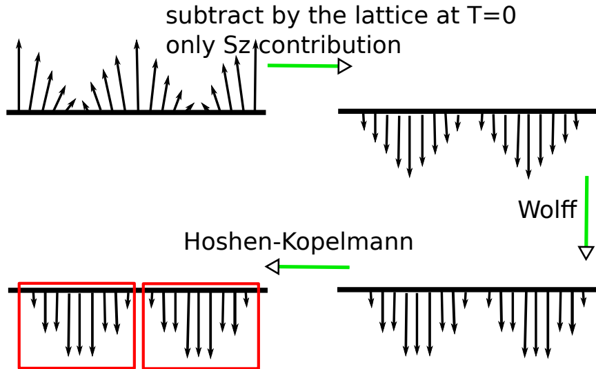
Fig. 2. The successive steps in the application of the algorithm by Wolff to the case of Heisenberg spin. See text for explanation.
