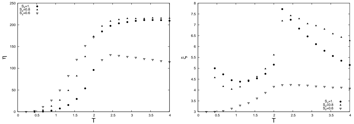
FIG. 9: Left : Number of clusters, Right : Average size of clusters, versus temperature for several values of S_z and for magnetic field B = 1.5 .
