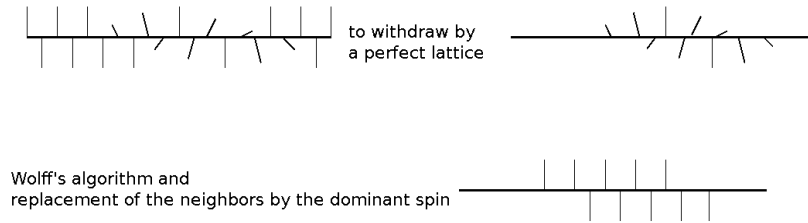
FIG. 2: Application of the algorithm by Wolff.
