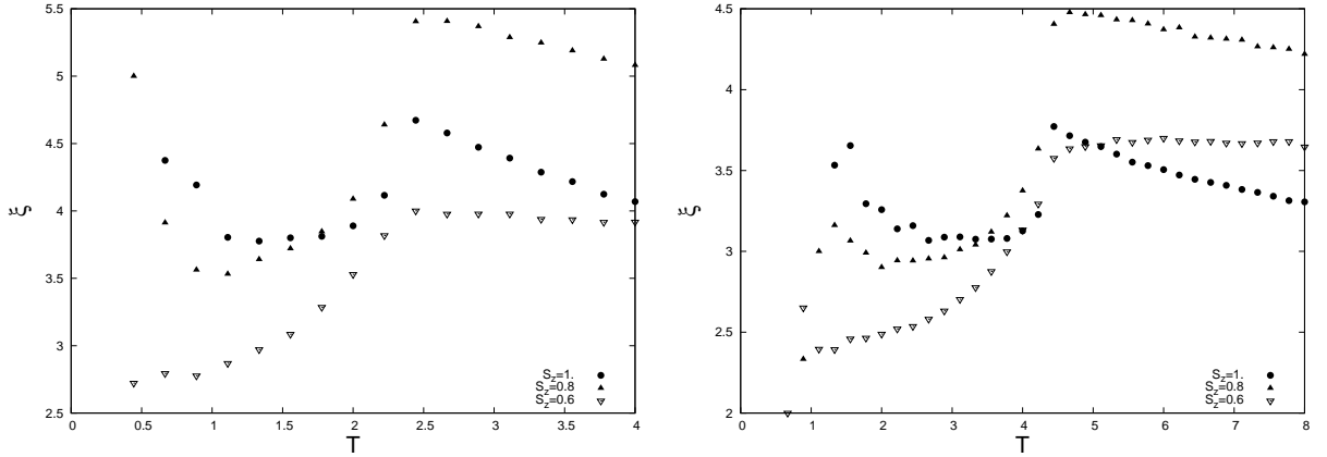
FIG. 4: Average size of clusters versus temperature for several values of S_z indicated on the figure and for anisotropy A = 0.01 (left) and A = 1 (right).
