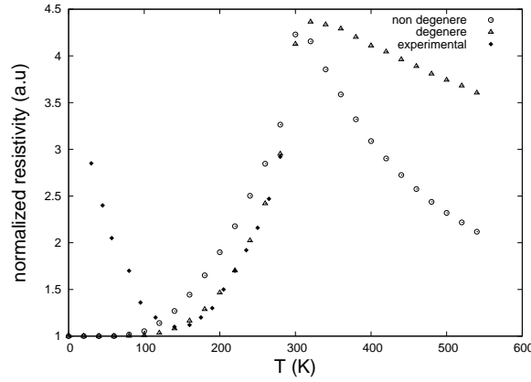
FIG. 14: Normalized spin resistivity versus temperature in MnTe : theoretical non-degenerate case (circles), theoretical degenerate case (triangles) and experimental results (diamonds) from Chandra et al. 39 See text for comments.
