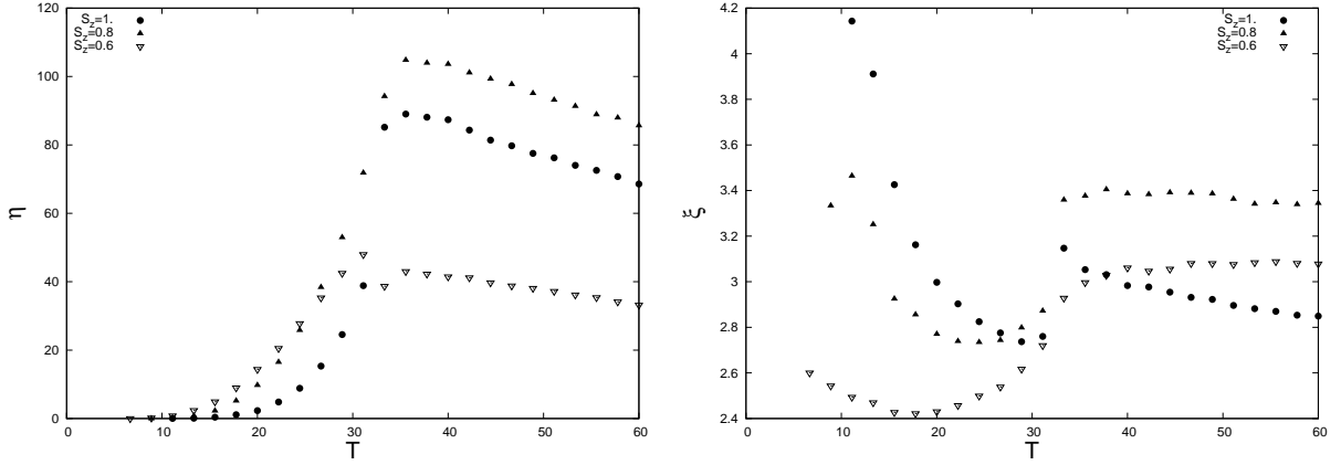
FIG. 13: Number of clusters (left) and cluster size (right) versus temperature T for MnTe structure obtained from Monte Carlo simulations.
