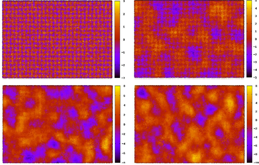
FIG. 1: Energy map of an itinerant spin in the xy plane with D_1 = 2 in unit of the lattice constant a and A = 0.01 , for T = 0.01 , T = 1.0 , T = 2.0 and T = 2.5 (from left to right, top to bottom, respectively).
