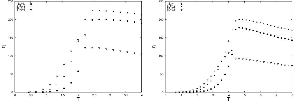
FIG. 3: Number of clusters versus temperature for anisotropy A = 0.01 (left), A = 1 (right). The values of S_z are indicated on the figure.
