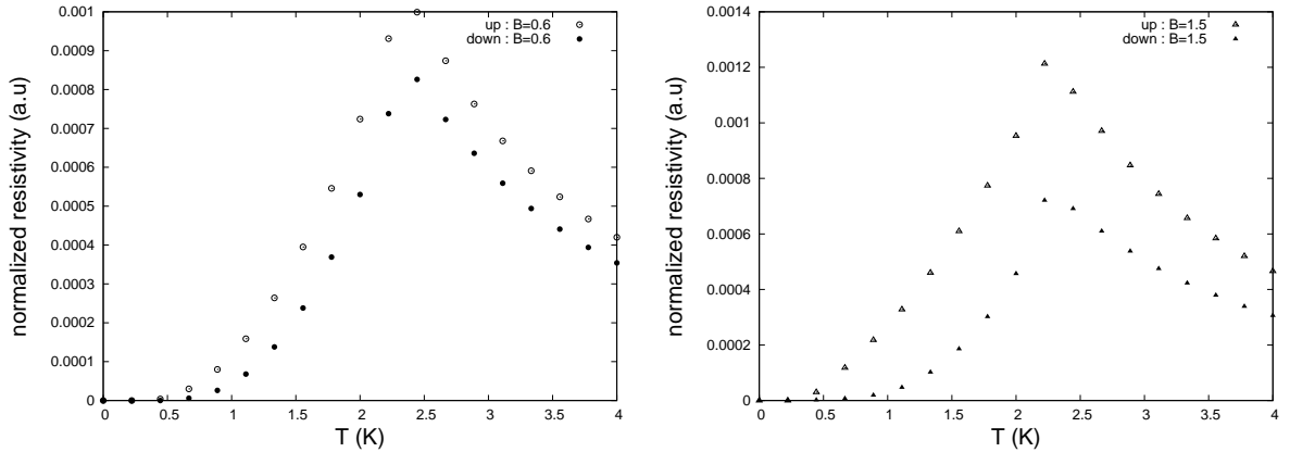
FIG. 11: Resistivities of up and down spins versus temperature for two magnetic field's strengths in the non degenerate case. Left (right) : B = 0.6(1.5) .
