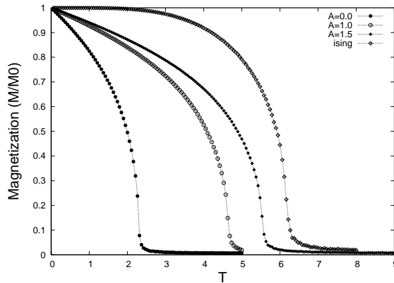
FIG. 6: Sublattice magnetization versus temperature for several values of anisotropy A .
