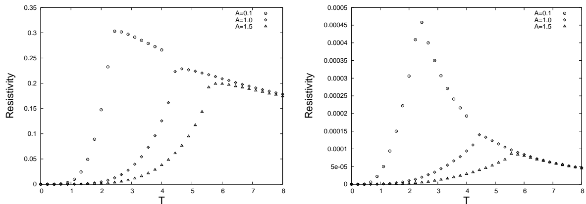
FIG. 7: Spin resistivity versus temperature for several anisotropy values A in antiferromagnetic BCC system. Left (right) curves : degenerate (non degenerate) system.
