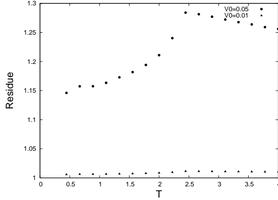
FIG. 5: Ratio \rho(\text{Born2})/\rho(\text{Born1}) versus temperature for V_0=0.05 (circles) and 0.01 (triangles). See text for comments.
