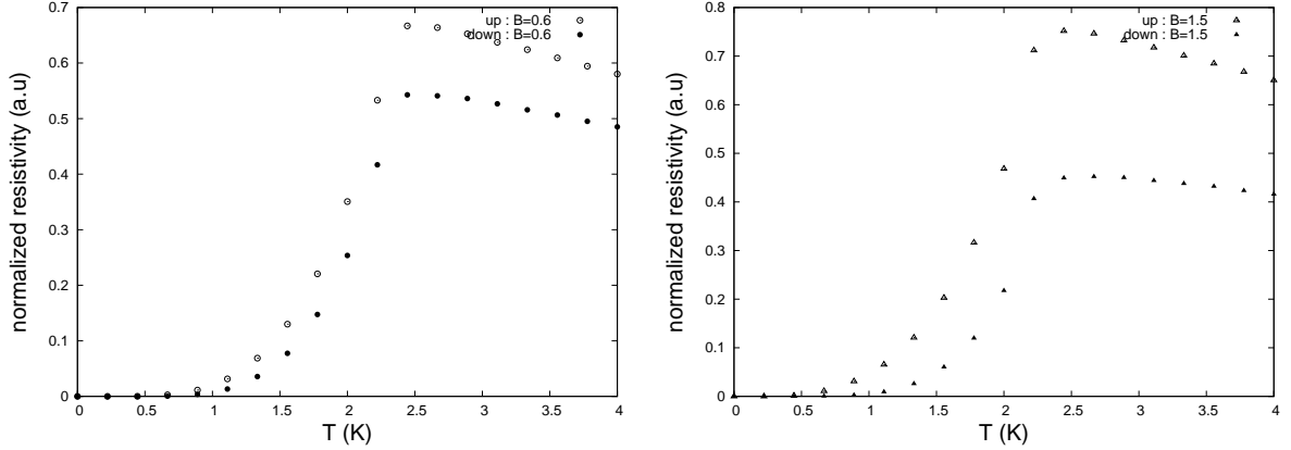
FIG. 10: Resistivities of up and down spins versus temperature for two magnetic field's strengths in the degenerate case. Left (right) : B = 0.6(1.5) .
