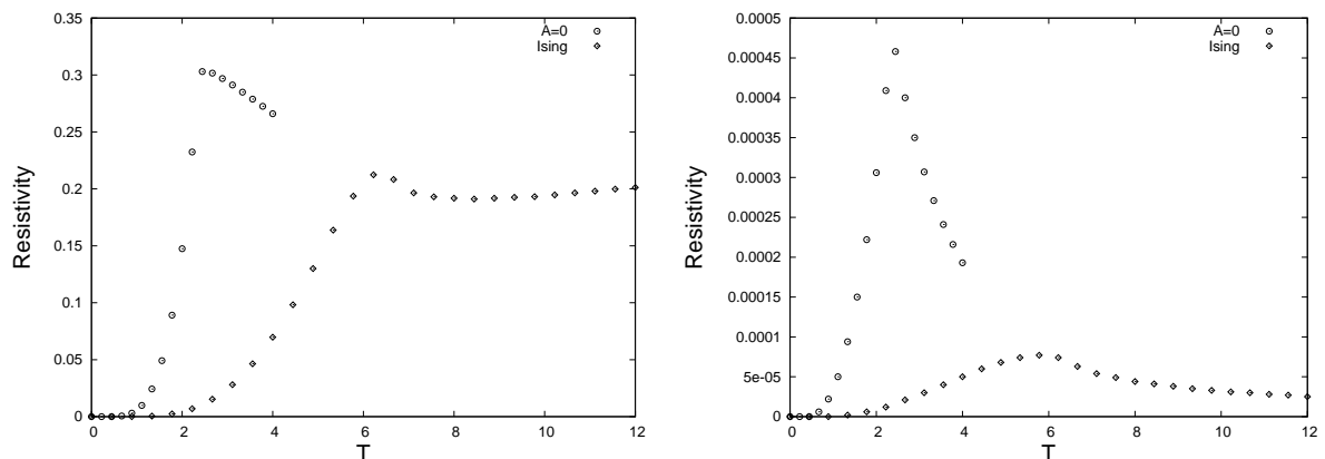
FIG. 8: Spin resistivity for pure Heisenberg and Ising models in antiferromagnetic BCC system. Left (right) curves : degenerate (non degenerate) system.
