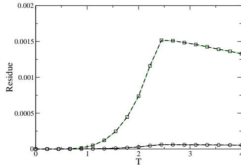
FIGURE 5: Ratio Residue= \rho(\text{Born2})/\rho(\text{Born1}) versus T for V_0=0.05 (squares, upper curve) and 0.01 (circles, lower curve). See text for comments.
