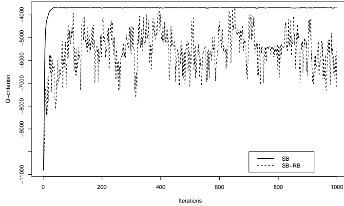
(a) Q-criterion of the first 1,000 iterations performed with the SB and the SB-RB algorithms
