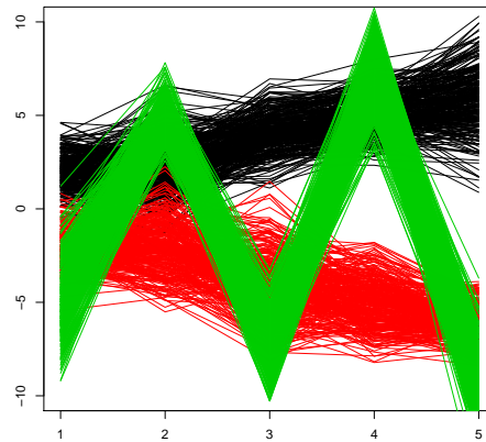
(b) Parallel coordinates of the optimal partition obtained with the SB or the RB-SB algorithm
