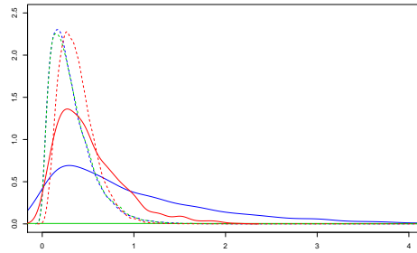
Figure 2: Densities of the \text{Gamma}(a_\gamma, b_\gamma) prior (solid line) and the posterior (dashed line) distributions of the parameter \gamma . Red line: (a_\gamma, b_\gamma) = (2, 4) , blue line: (a_\gamma, b_\gamma) = (1, 1) , green line: (a_\gamma, b_\gamma) = (0.01, 0.01) , prior densities are plotted in logarithmic scale.
