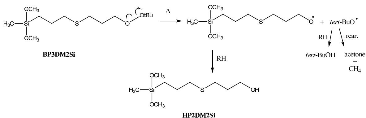
Figure 10. Decomposition of BP3DM2Si .
