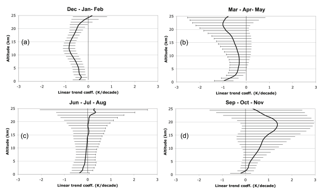
Fig. 6. Seasonal linear trends profiles at Dumont d'Urville, as derived from the AMOUNTS model by averaging the three corresponding monthly mean temperatures for (a) summer, (b) autumn, (c) winter and (d) spring. One-sigma uncertainty estimations are shown.
