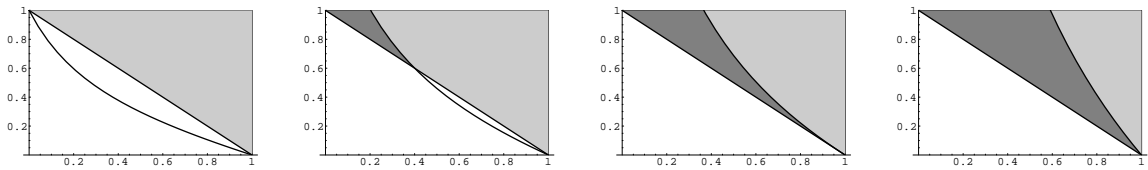
FIGURE 1. Plot of the admissible regions (gray areas) with symmetry breaking region established in Theorem 7 (dark grey) in (\eta, \theta) coordinates, with \eta := b - a , for various values of a , in dimension d = 3 : from left to right, a = 0 , a = -0.25 , a = -0.5 and a = -1 . The two curves are \eta \mapsto \vartheta(p, d) = 1 - \eta and \eta \mapsto \Theta(a, p, d) , for p = 2d/(d - 2 + 2\eta) . In the range a \in (-1/2, 0) , they intersect for a = a_-(p) , i.e. \eta = 2a(1 - d)/(d + 2a) . They are tangent at (\eta, \theta) = (1, 0) for a = -1/2 . The symmetry breaking region contains a cone attached to (\eta, \theta) = (1, 0) for a < -1/2 , which determines values of \gamma for which symmetry breaking occurs in the logarithmic Hardy inequality.
