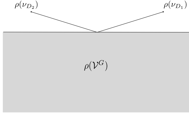
Figure 2: The combinatorial data attached to X_0
