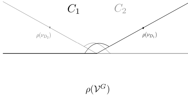
Figure 3: The colored fan \mathcal{E} .
