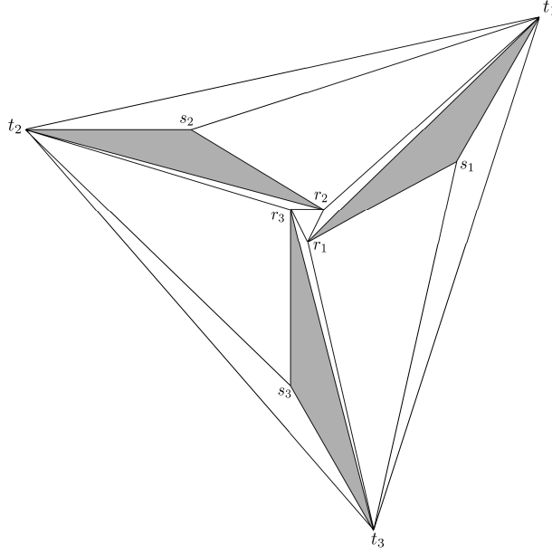
Figure 1: The fans \mathcal{E} (grey) and \mathcal{E}_0 .
