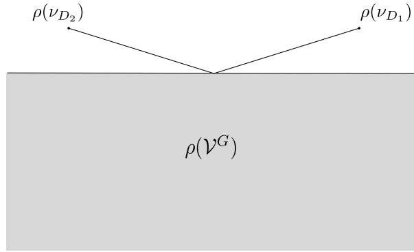
Figure 2: The combinatorial data attached to X_0
