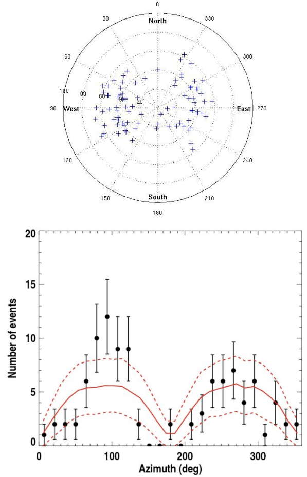
Figure 9: Sky map of the events observed by the small NS oriented antennas (top). Azimuthal distribution of events measured by the NS antenna mini-array (bottom). Definitions of the lines are similar to those in the figure 8.
