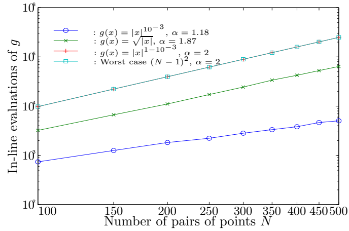
FIGURE 1. Number of in-line evaluations with respect to the number of pairs, for various cost functions. The number \alpha is the slope of the log-log graphs.
