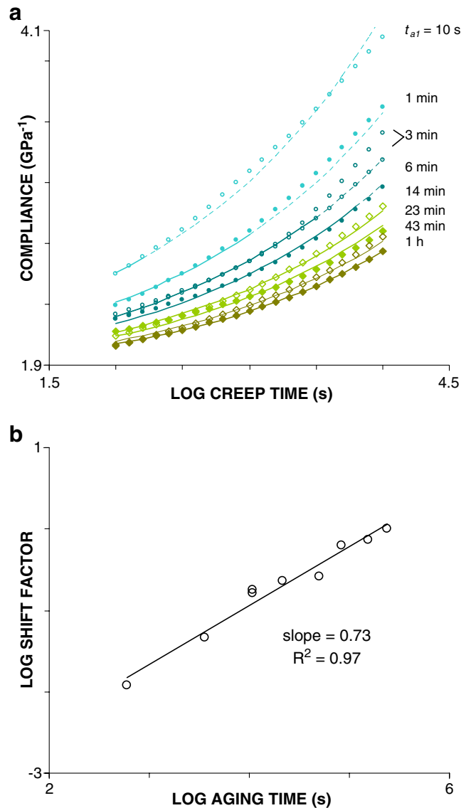
Fig. 9 Model fitting based on Eq. 3 applied on Nakano's data: a Agreement between experimental and modelled creep curves for fitting 1. Solid lines represent the prediction for values of t_c < t_a/3 ; dashed lines correspond to modelled values not satisfying the snapshot condition t_c > t_a/3 . b Relationship between shift factors a and aging times t_a in double logarithmic scale
