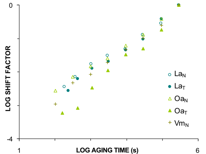
Fig. 6 Model fitting based on Eq. 4. Relationship between shift factors a and aging times t_a in double logarithmic scale for different samples
