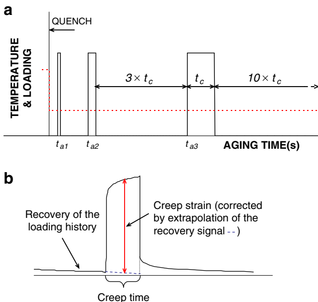
Fig. 1 Experimental procedure for investigating the aging time effect on small strain creep properties. a Loading schedule: dashed line , temperature; solid line , load. t_a aging time, t_c creep time. b Accounting for the correction of the creep signal. Dashed line , extrapolation of the recovery signal to the creep test duration
