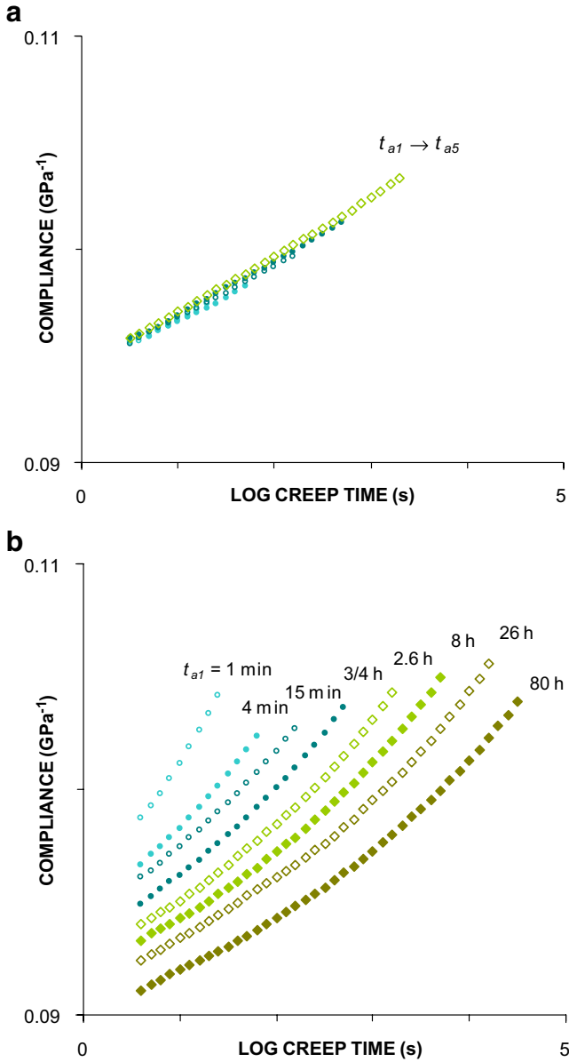
Fig. 3 Evidence of physical ageing occurrence in green wood (sample Vm N ). a Set of creep tests performed at different elapsed times t_1 – t_5 counting from the onset of the test without preliminary heating above T_g . b Set of creep tests performed on the same sample at different aging times t_{a1} – t_{a8} following the quench
