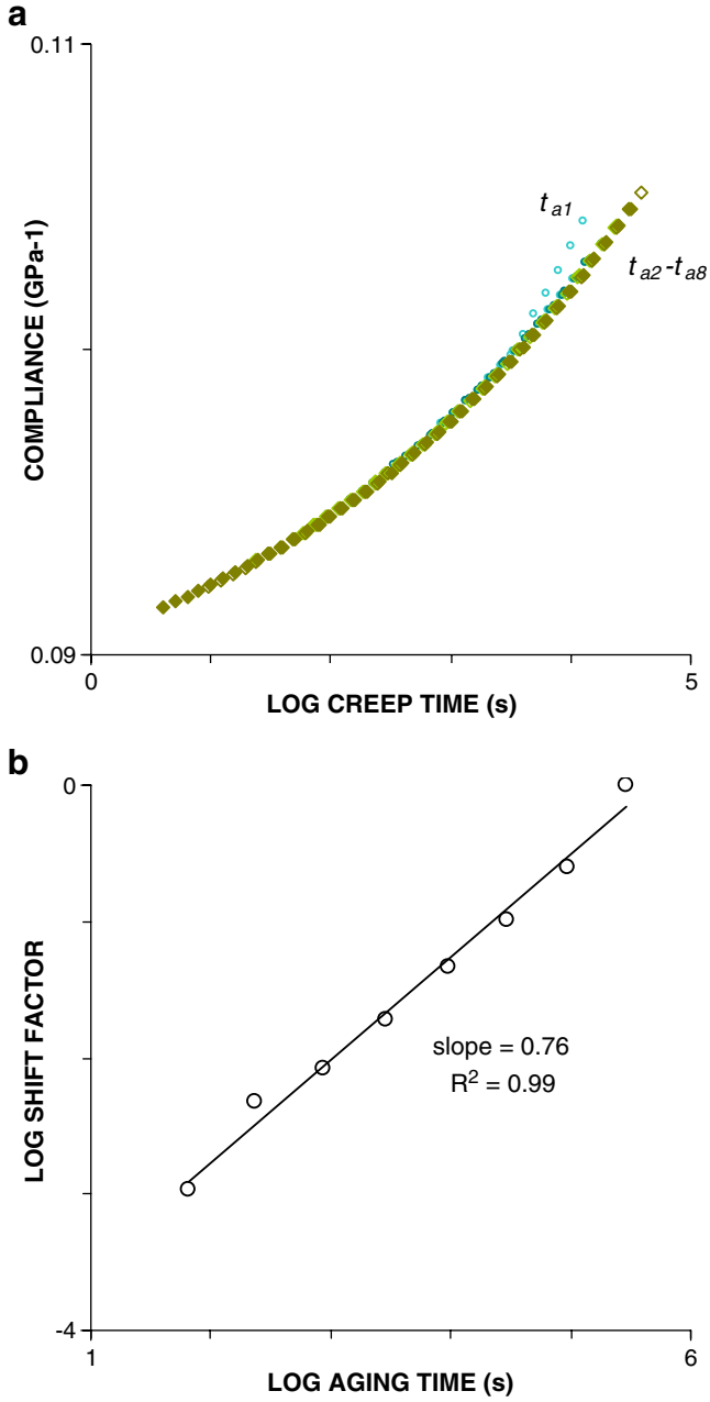
Fig. 4 Relationship between retardation and ageing time based on visual assessment (sample Vm N ). a Master curve obtained by visual shifting of individual creep curves from Fig. 3b. b Double logarithmic plot of shift factors a versus the aging time t_a
