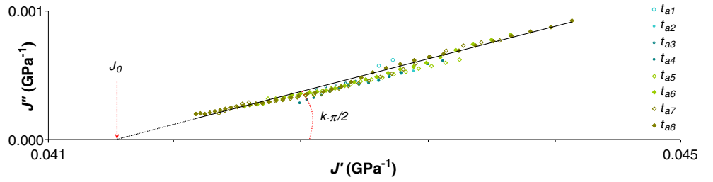
Fig. 5 Complex plot of a sequence of creep tests performed at different aging times t_a after the quench where J' is storage compliance and J'' delayed compliance (sample Oa N ). For signification of J_0 and k , see in the text
