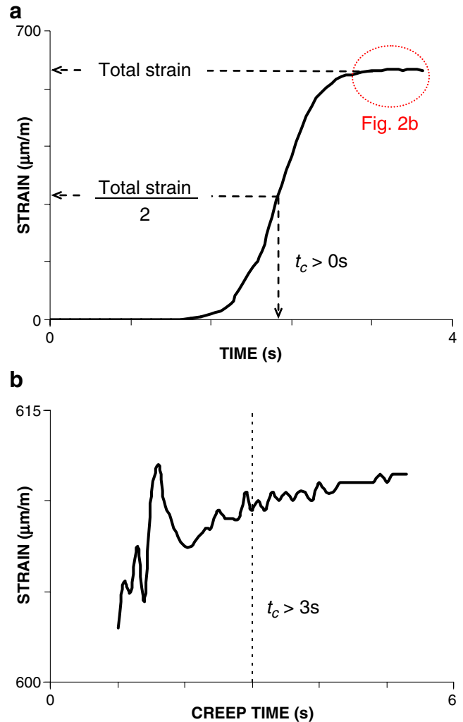
Fig. 2 a Method to determine the point considered as the start of the loading. b Zoom on the zone of the very first seconds following the loading (unsmoothed data). t_c testing time
