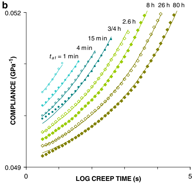
Fig. 7 Example of model fitting based on Eq. 4 for sample O_{a_N} : a Master curve produced by shifts resulting from optimisation without any presumed dependency between doubling and aging times. b Example of agreement between experimental ( dots ) and modelled creep curves ( lines ). Creep curve corresponding to the aging time t_{a8} = 3.3 days was taken as a reference
