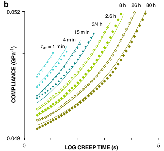
Fig. 8 Example of model fitting based on Eqs. 4 and 5 for sample O_{a_N} : a Master curve produced by shifts resulting from optimisation accounting for linear logarithmic dependency between doubling time and aging time. b Example of agreement between experimental and modelled creep curves issued from fitting 2. t_a aging time
