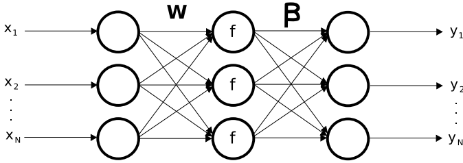
Fig. 4. Structure of a classical Single Layer Feedforward Neural Network (SLFN). The input values (the data) \mathbf{X} = (\mathbf{x}_1, \dots, \mathbf{x}_N) are weighted by the \mathbf{W} coefficients. A possible bias \mathbf{B} (not on the figure) can be added to the weighted inputs \mathbf{w}_i \mathbf{x}_i . An activation function f taking this weighted inputs (plus bias) as input is finally weighted by output coefficients \beta to obtain the output \mathbf{Y} = (\mathbf{y}_1, \dots, \mathbf{y}_N) .
