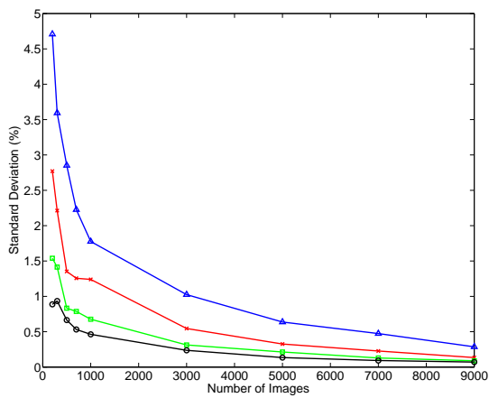
(e) OutGuess
