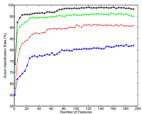
(f) StegHide
