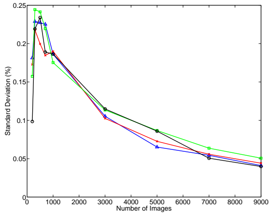
(a) F5
