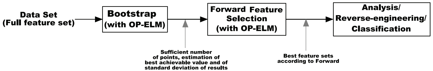
Fig. 3. Schematic view of the proposed methodology: (1) An appropriate number of data samples to work with is determined using a Bootstrap method for statistical stability; (2) The forward selection is performed using an OP-ELM classifier to find a good features set. Follows a possible interpretation of the features or the typical classification for steganalysis.
