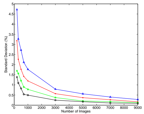
(f) StegHide
