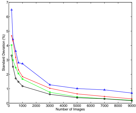
(c) MBSTEG
