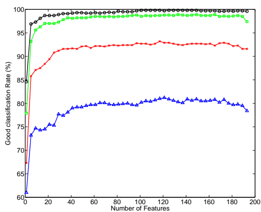
(e) OutGuess
