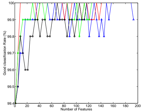
(a) F5
