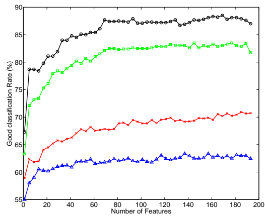
(c) MBSTEG
