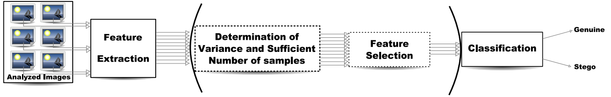
Fig. 1. Overview of the typical global processing for an analyzed image: features are first extracted from the image and then processed through a classifier to decide whether the image is cover or stego. In the proposed processing is added an extra step aimed at reducing the features number and having an additional interpretability of the steganalysis results, by doing a feature selection.
