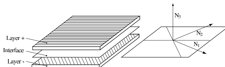
Figure 2: Orthotropic directions of the interface
