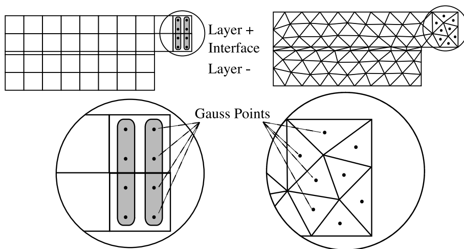
Figure 3: Regular (left) and unregular (right) mesh (grey area: Integration point aligned in the thickness)
