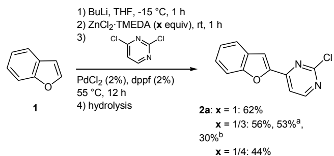
Scheme 1 a Using PPh 3 (4 mol.%) instead of dppf. b Using PCy 3 (4 mol.%) instead of dppf.
